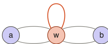
Figure 7: After identifying u and v as w
