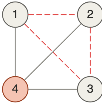
Figure 28: K_4 , triangle dashed
